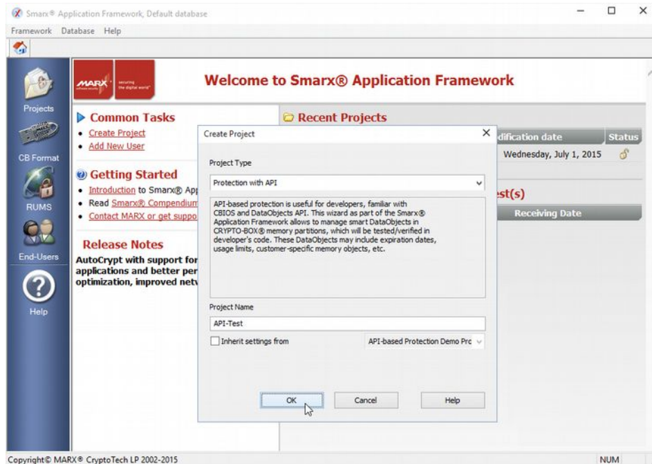
Fig. 4.3: Creating a new API-based project
