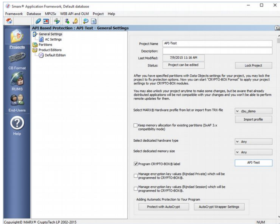
Fig. 4.4: API-based project: project settings
