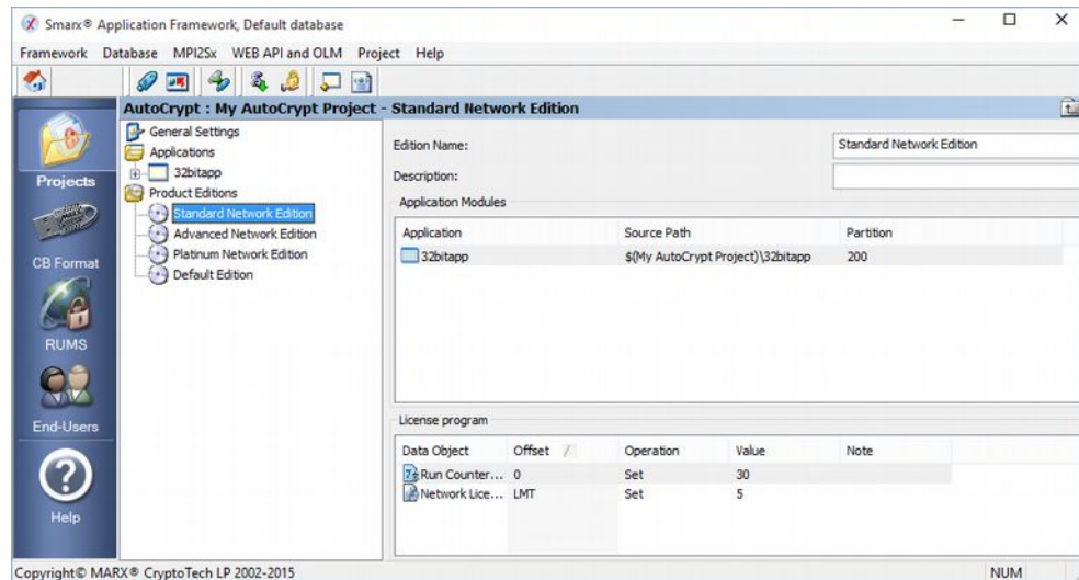
Fig. 4.17: Adding Product Editions
